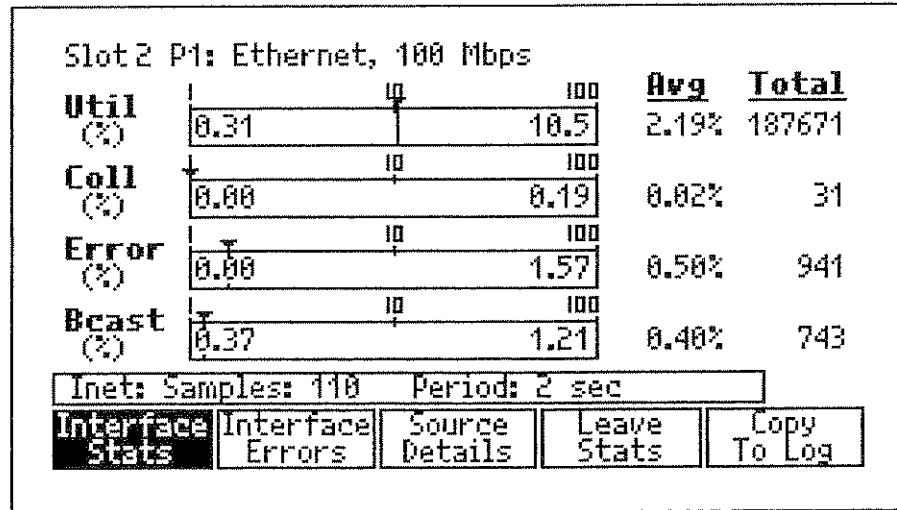
Figure 9-9. MultiPort Statistics Interface Stats
