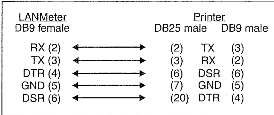
Figure 14-8. Printer Cable Connections
