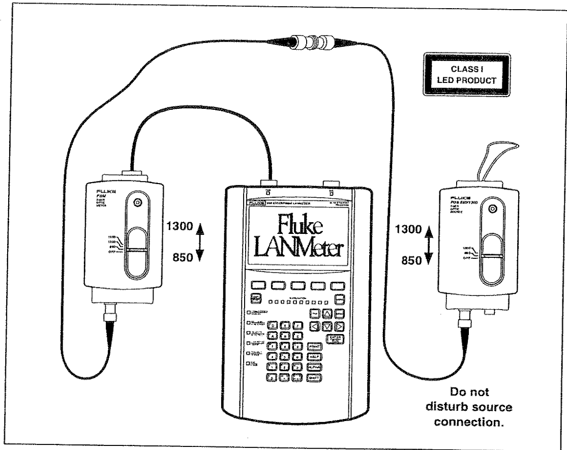
Figure 4-2. Connections for Setting a Reference Level
