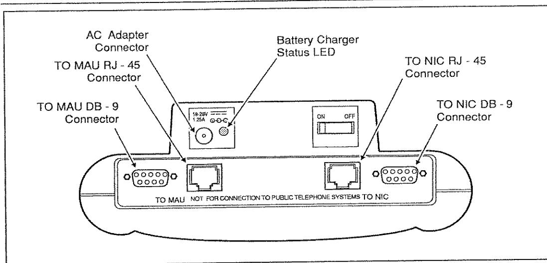
Figure 3-11. Network and AC Adapter Connectors (680 Shown)
