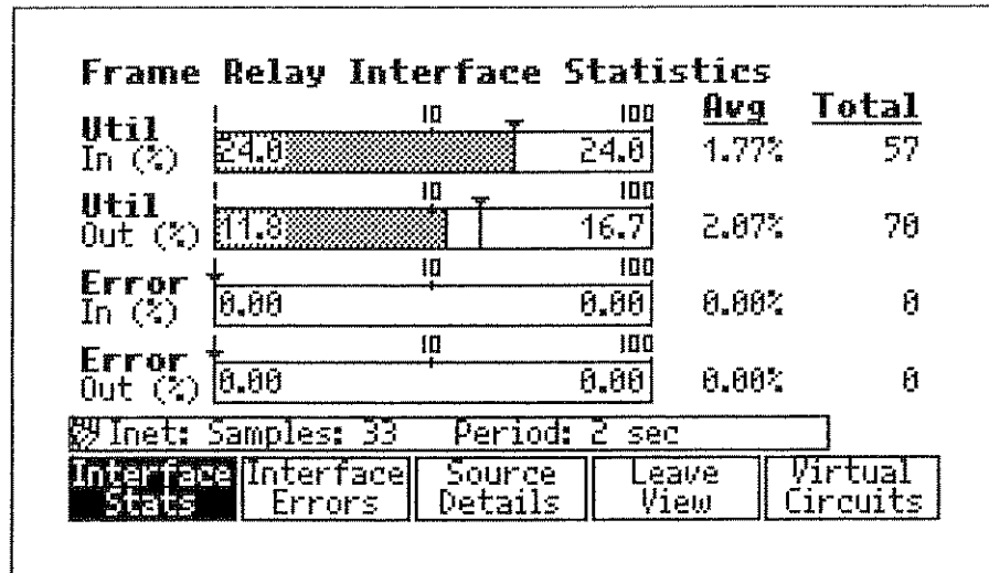
Figure 12-5. Frame Relay Interface Statistics Sample Results
