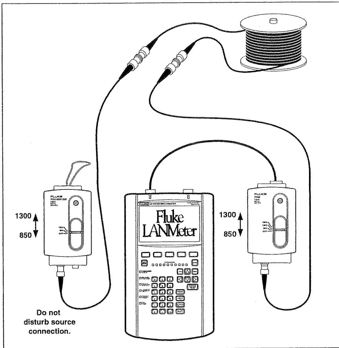
Figure 4-3. Connections for Measuring Optical Loss
