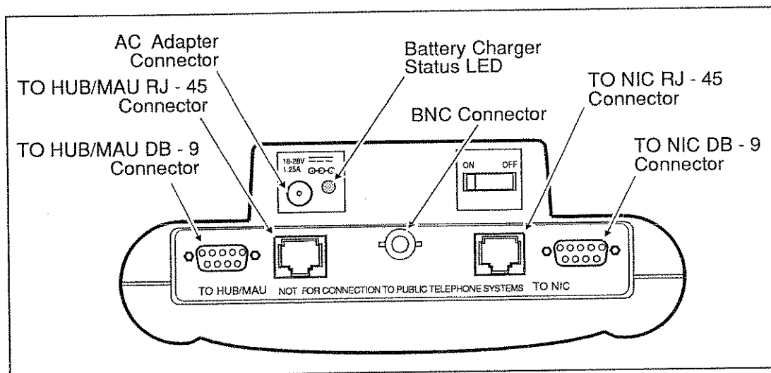
Figure 2-2. Network and AC Adapter Connectors (686/685 Shown)
