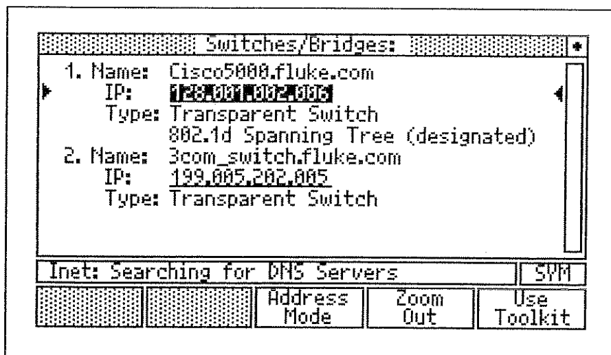
Figure 9-4. Switches and Bridges Results
