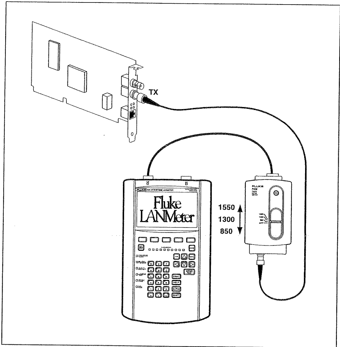
Figure 4-4. Connections for Measuring Output Power
