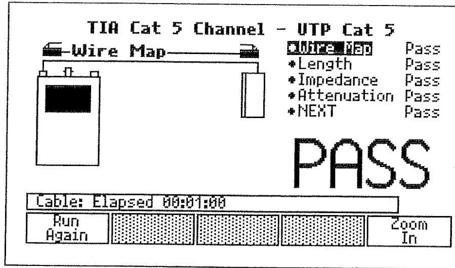
Figure 4-10. Cable Autotest Sample Results
