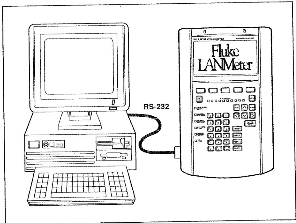
Figure D-10. Software Update and File Transfer Connection
