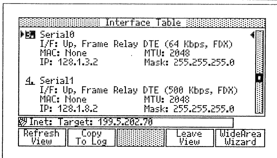
Figure 12-4. Frame Relay Interface Table Sample Results
