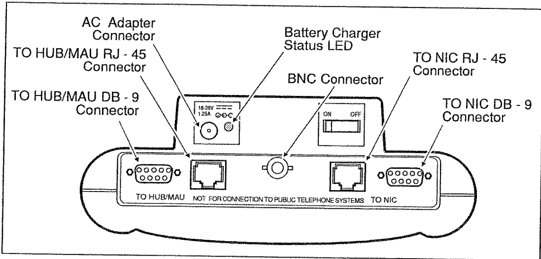
Figure 3-9. Network and AC Adapter Connectors (686/685 Shown)
