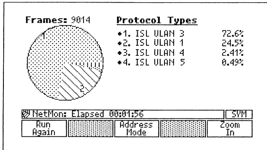
Figure 5-19. Protocol Mix (VLANs) Sample Results
