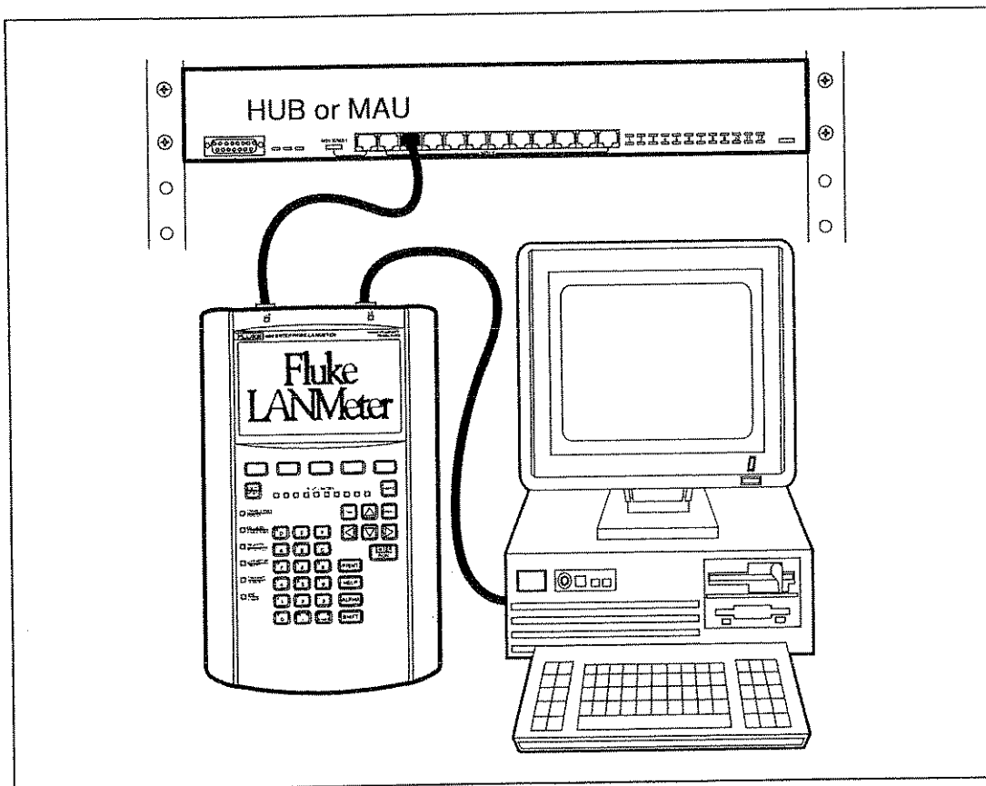
Figure 2-7. Expert-T Autotest Connections
