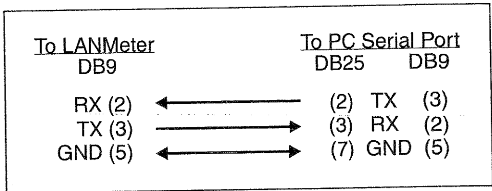
Figure D-11. Software Update and File Transfer Cable
