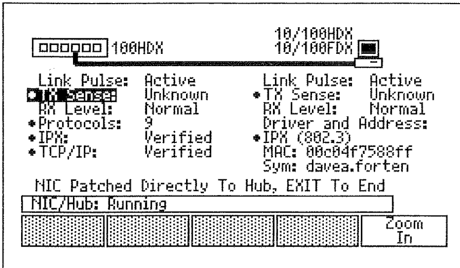
Figure 6-5. Ethernet Expert-T Autotest Sample Results
