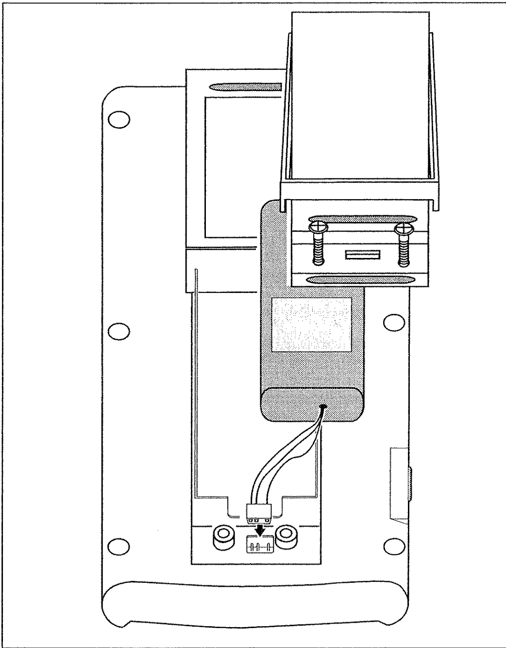
Figure C-1. Battery Replacement Exploded View
