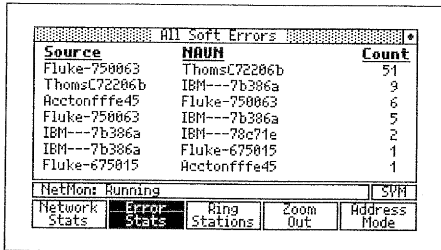
Figure 5-11. Token Ring Error Statistics Fault Domain Sample Results
