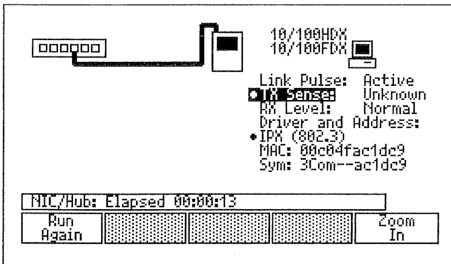
Figure 6-4. Ethernet NIC Autotest Sample Results
