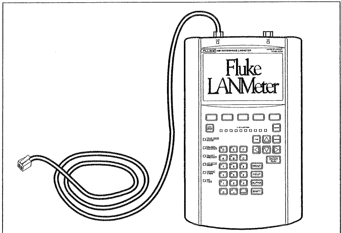
Figure A-5. Bad Cable Test Connection
