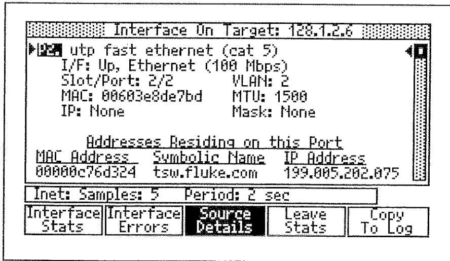
Figure 9-8. MultiPort Statistics Source Details
