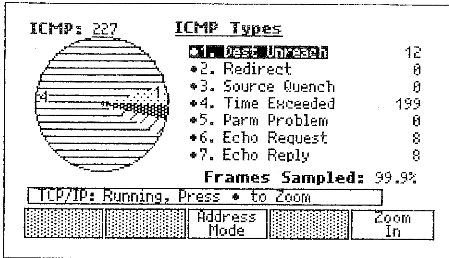
Figure 8-24. ICMP Monitor Sample Results
