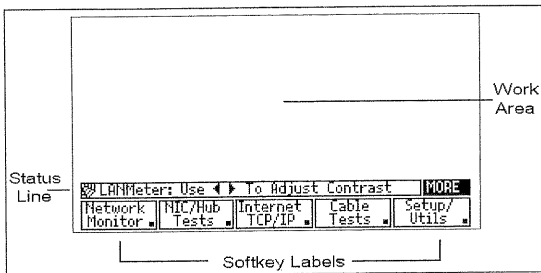
Figure 3-2. LCD Display Areas
