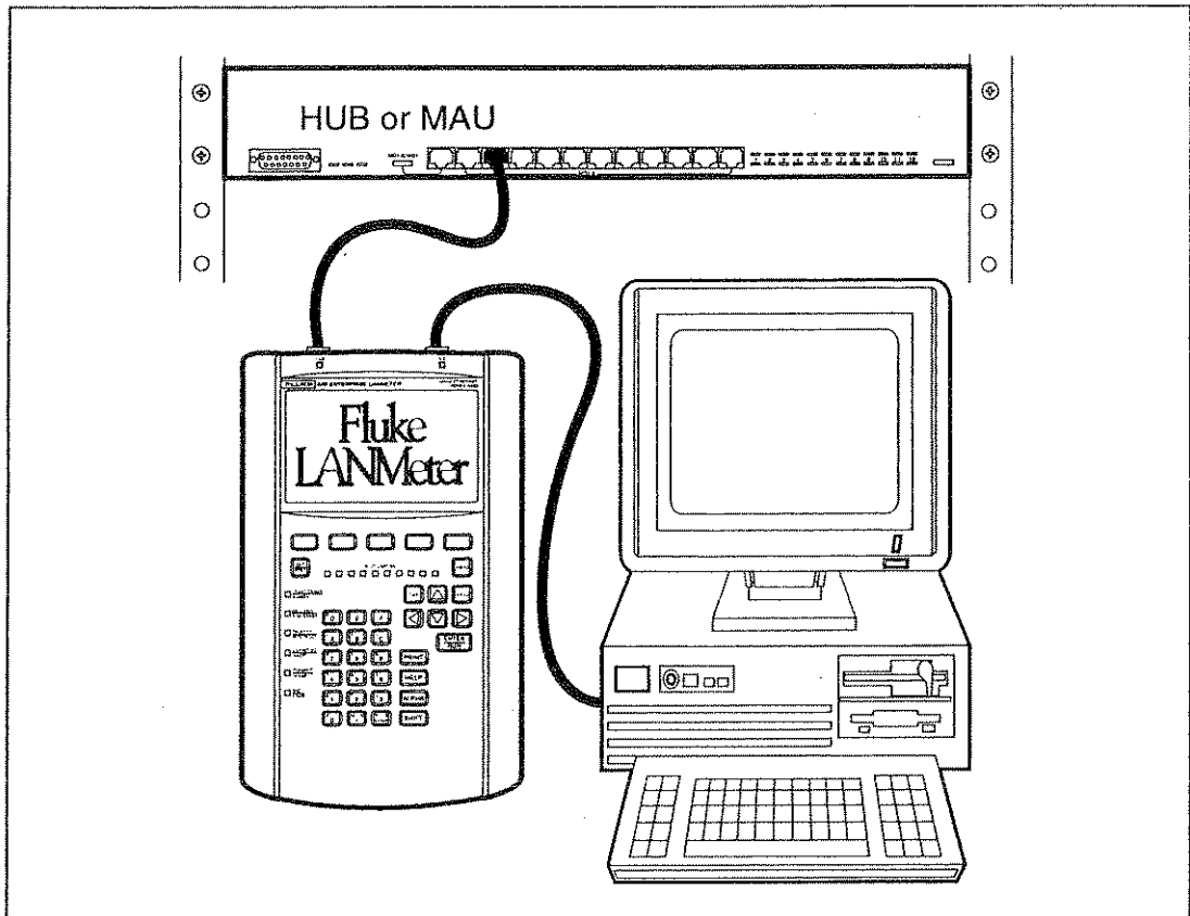
Figure A-4. Expert-T Autotest Connections
