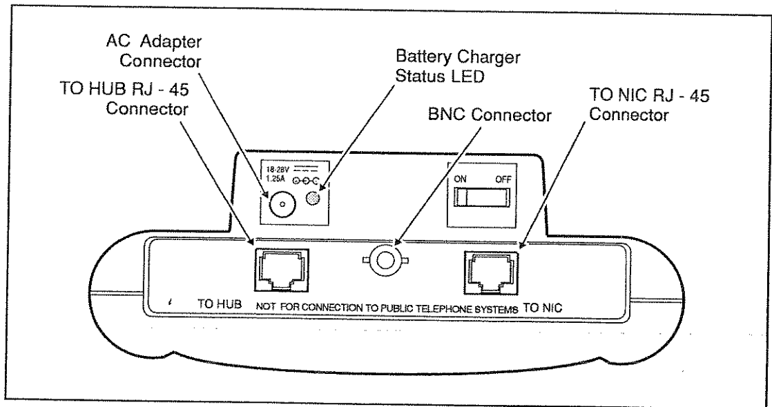
Figure 3-10. Network and AC Adapter Connectors (683/682 Shown)
