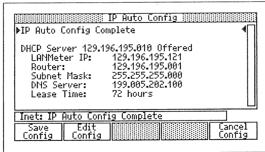
Figure 8-8. IP Auto Config (DHCP Mode) Results Screen
